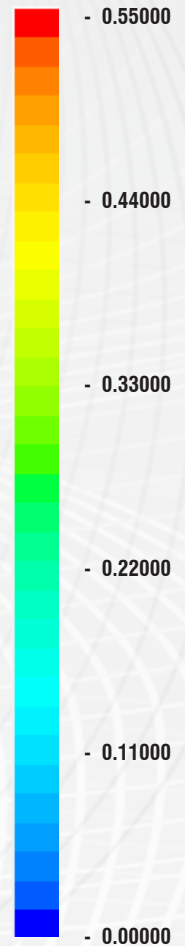
Mole Fraction of CH 4
